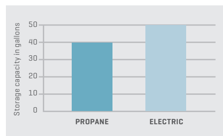
CHART 1 STORAGE TANK SIZE NEEDED FOR 70 GALLON FIRST HOUR DELIVERY
