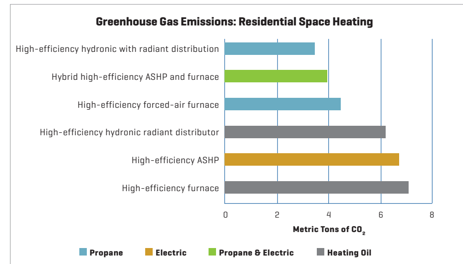
Source: Newport Partners 2013 Heating Study. Lower numbers represent lower greenhouse gas emissions. Findings are national averages based on computer energy simulations of a typical new home across 20 locations in warm, moderate, and cold climate zones.
